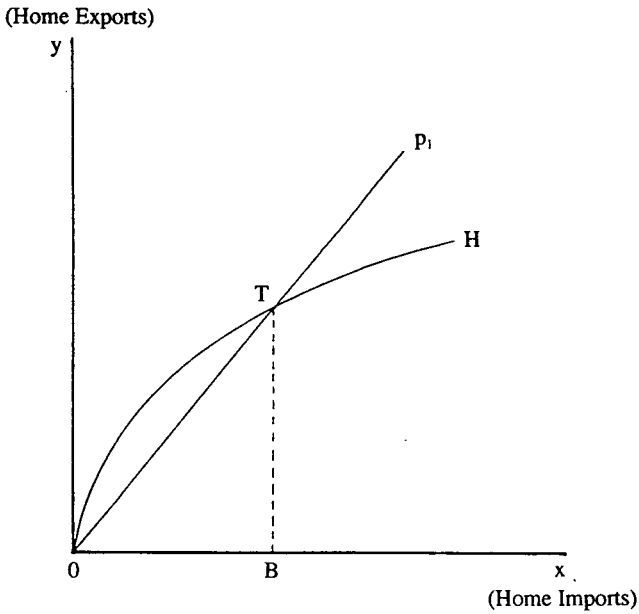
FIGURE 6 Offer Curve
