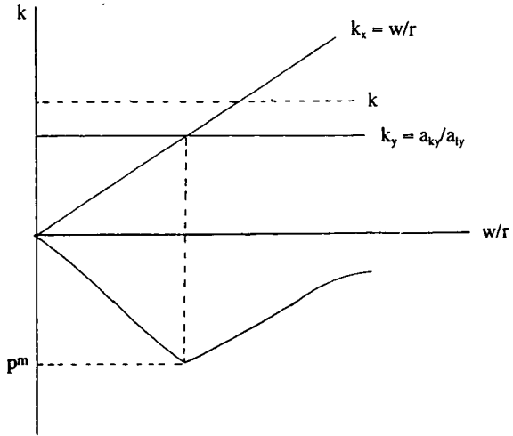
FIGURE 3 Harrod-Johnson Diagram
